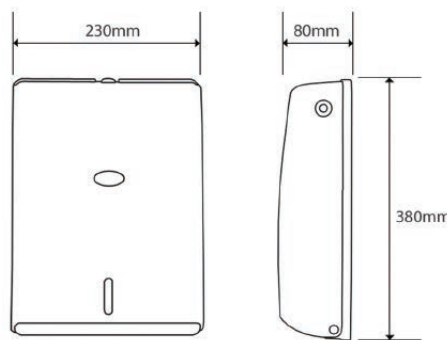
HD/35 Compact Paper Towel Dispenser
