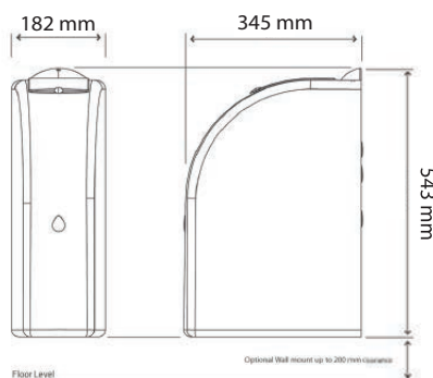
SW/03 Femcare Sanitary Bin Sensor
