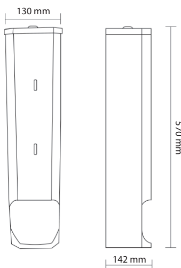
TR/05 white epoxy Toilet Roll dispenser
